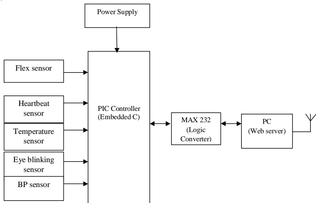
Fig. 3.1 Block diagram of the project
