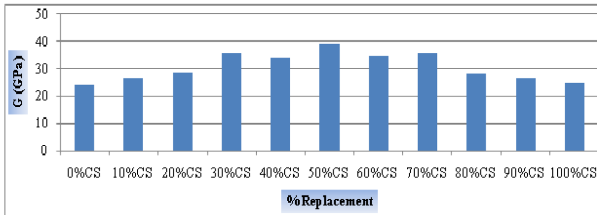
Chart 5. Modulus Of Elasticity ( E ) Vs. % Replacement
