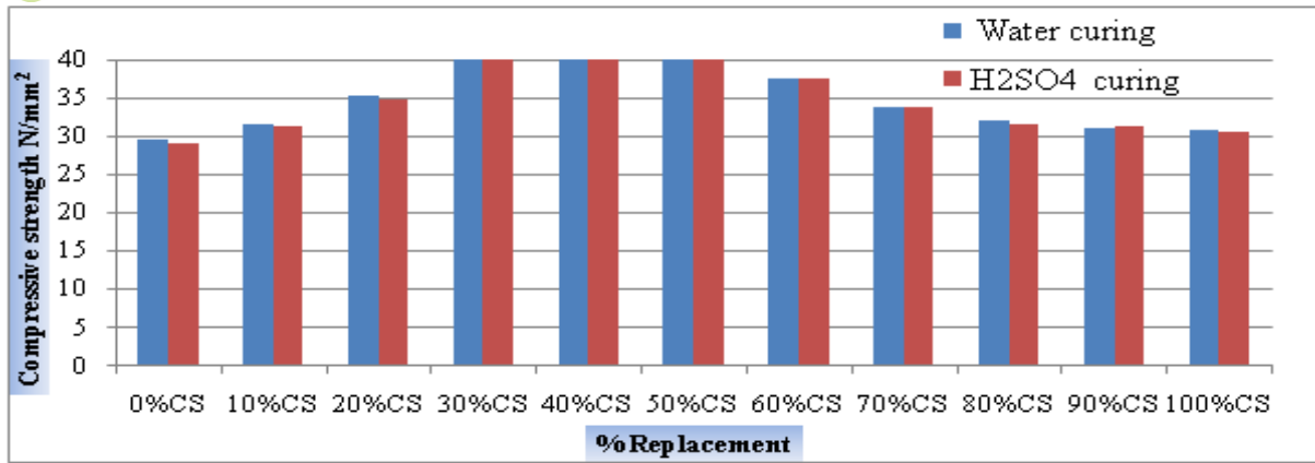
Chart 3. Compressive Strength(H 2 SO 4 ) Vs. % Replacement
