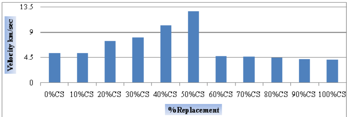
Chart 4. Pulse Velocity Vs. % Replacement
