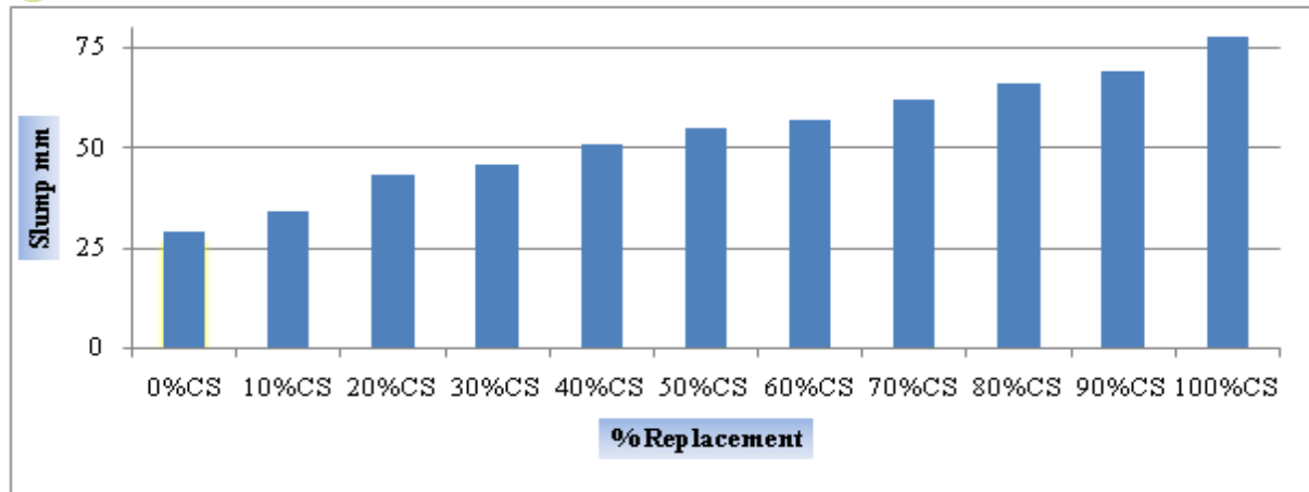
Chart 2. Slump Vs. % Replacement
