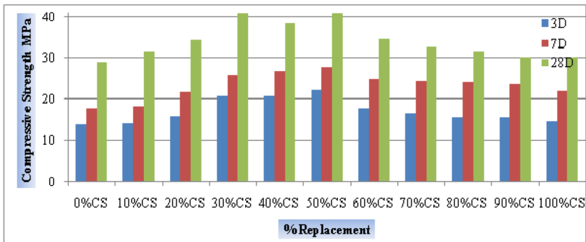
Chart 1. Compressive Strength (N/mm 2 ) Vs. % Replacement
